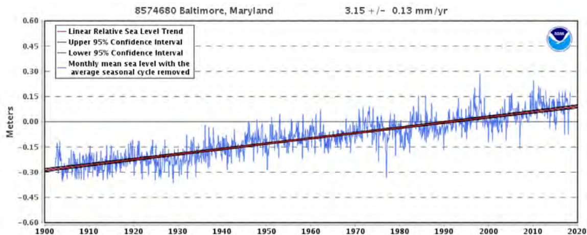
Figure 6.11. Tide gauge measurements at Baltimore, MD, obtained from NOAA (downloaded 8/2/18). https://tidesandcurrents.noaa.gov/sltrends/ .
