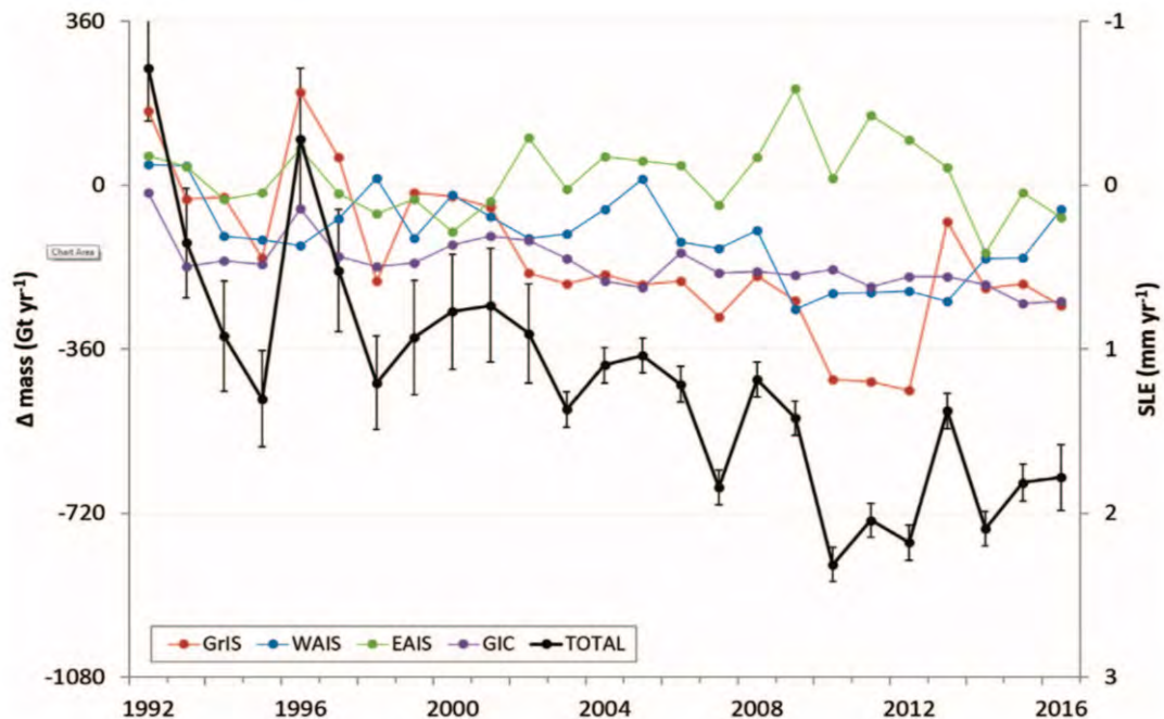
Figure 4.5: Annual time series of mass trends (sea level equivalent, SLE) for the Greenland Ice Sheet (GrIS), West Antarctic Ice Sheet (WAIS), East Antarctic Ice Sheet (EAIS), glaciers and ice caps (GIC). Bamber et al. (2018)
