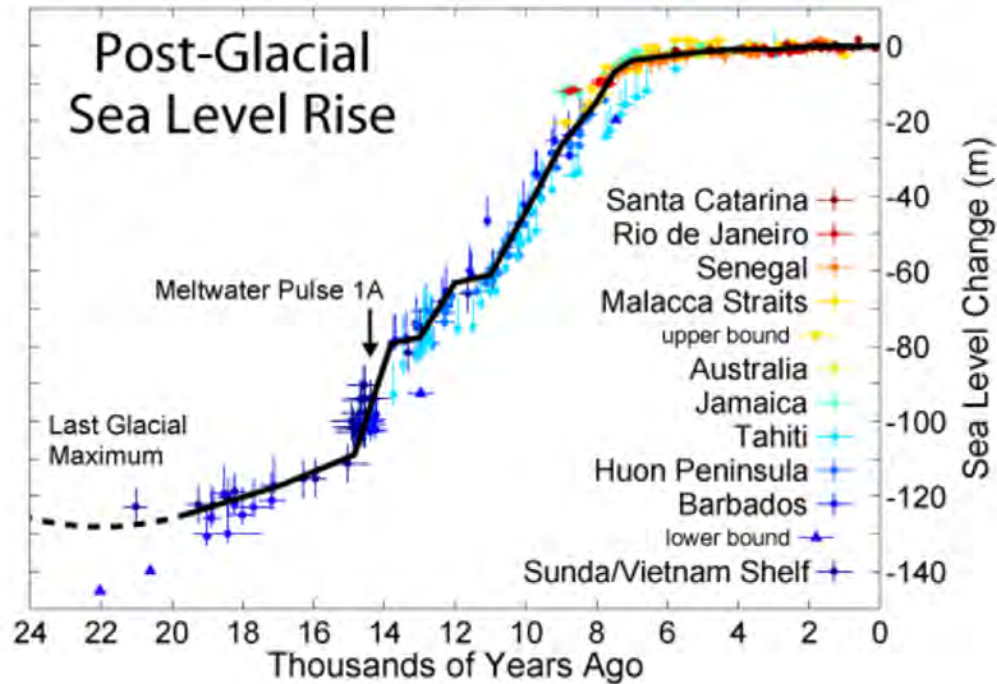
Figure 3.1 Estimated global sea level changes since the Last Glacial Maximum (~21,000 years ago). This figure was prepared by Robert A. Rohde from published data, and is incorporated into the Global Warming Art project. https://commons.wikimedia.org/wiki/File:Post-Glacial_Sea_Level.png
