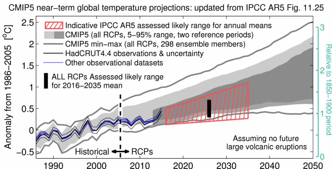
Figure 6. Comparison of CMIP5 climate model simulations of global surface temperature anomalies with observations through 2014 (HadCRUT4). Updated from Figure 11.25 of the IPCC AR5, to include observations through 2014. 25
