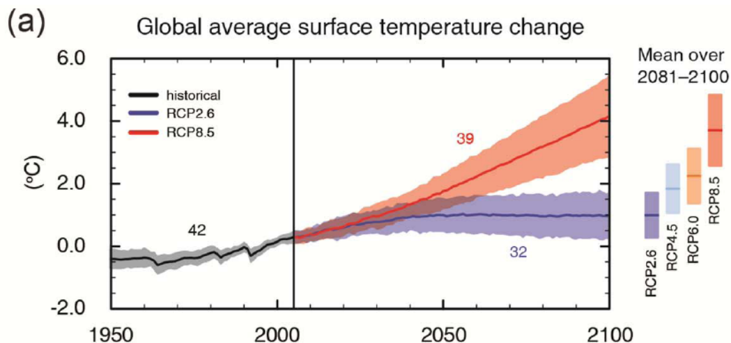
Figure 7: Figure SPM.7 of the IPCC AR5 WG1. CMIP5 multi-model simulated time series from 1950 to 2100 for change in global annual mean surface temperature relative to 1986–2005. Time series of projections and a measure of uncertainty (shading) are shown for scenarios RCP2.6 (blue) and RCP8.5 (red). Black (grey shading) is the modelled historical evolution using historical reconstructed forcings. The mean and associated uncertainties averaged over 2081–2100 are given for all RCP scenarios as colored vertical bars.
