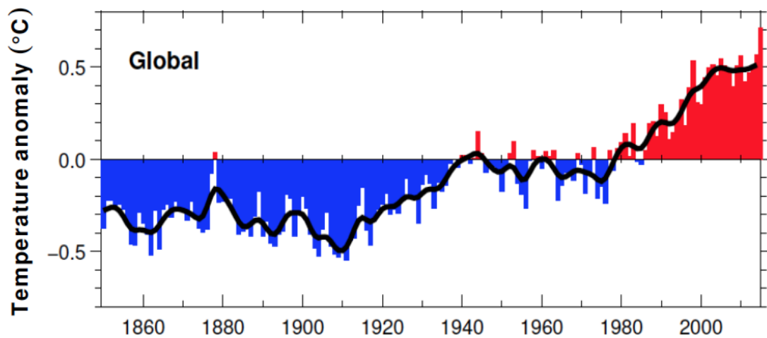
Figure 2: Global surface temperature anomalies from the UK HadCRUT4 dataset 19
