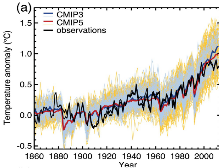
Figure 3. Comparison of the CMIP3 and CMIP5 simulations of global surface temperature anomalies with observations. Figure 10.1 from the IPCC AR5.
