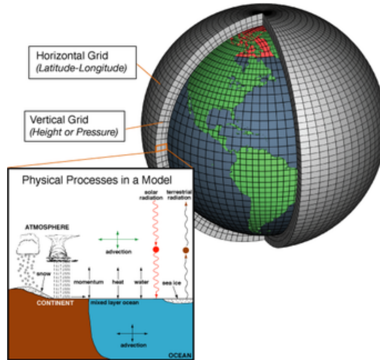
Figure 1. Schematic of a global climate model. 1
