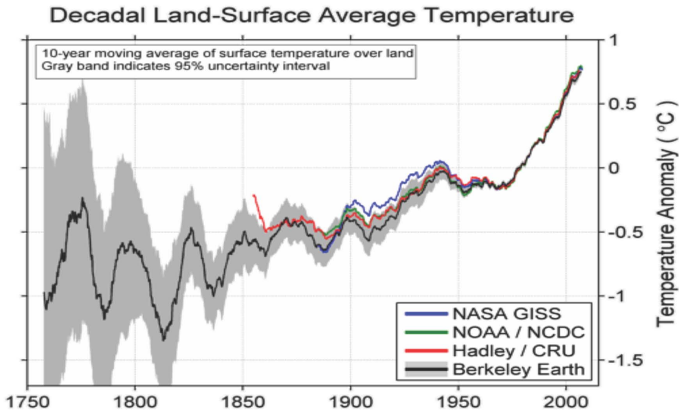
Figure 4: Global land surface temperature anomalies since 1750, smoothed with a 10 year filter. 21
